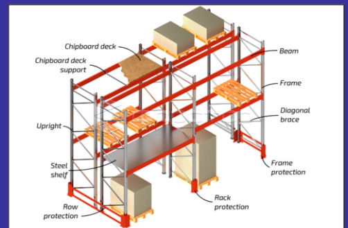
RACKING SYSTEM
